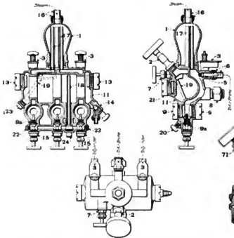
Figs. 3200-3202. Nathan Triple Feed Locomotive Lubricator. Nathau Manufacturing Co.
